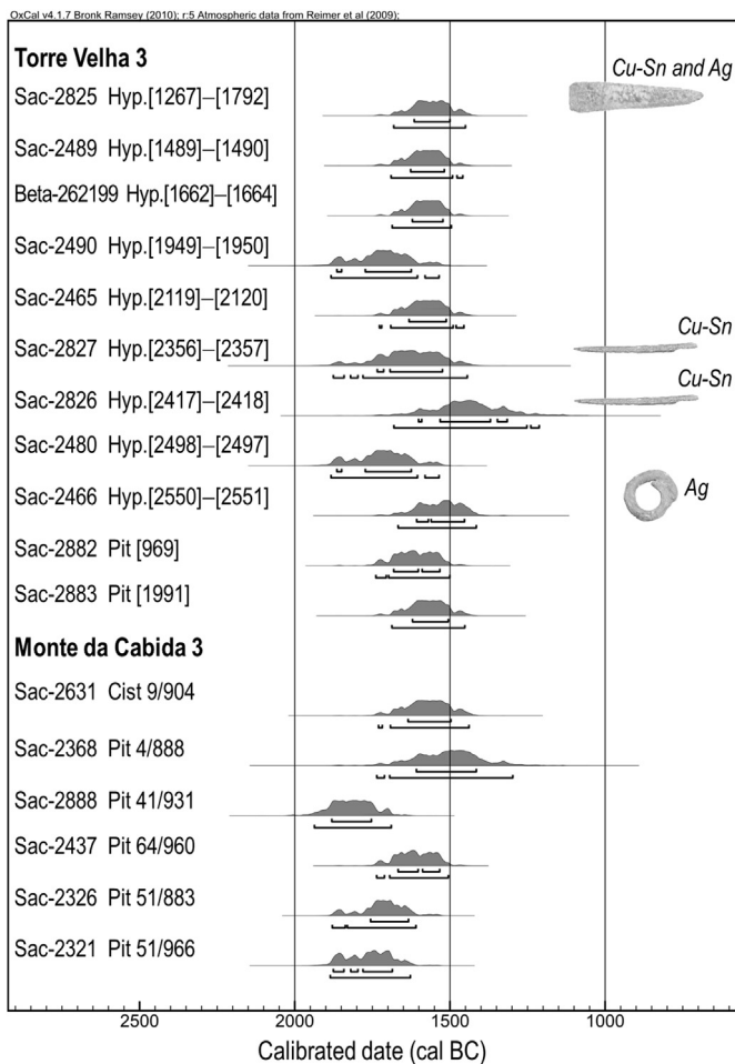
Fig. 7. Calibrated radiocarbon dates using the IntCal09 calibration curve (Reimer et al., 2009) and OxCal program (V4.1) (Bronk Ramsey, 2001, 2009) with indication of burials with bronze (Cu–Sn) and/or silver (Ag) artefacts.
