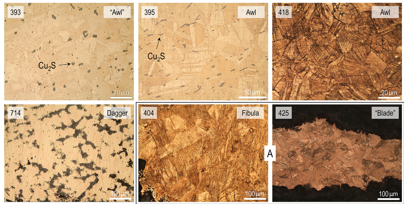
Fig. 5. Microstructures of MBA bronze artefacts from Torre Velha 3 (A: microstructures of Iron Age artefacts).
