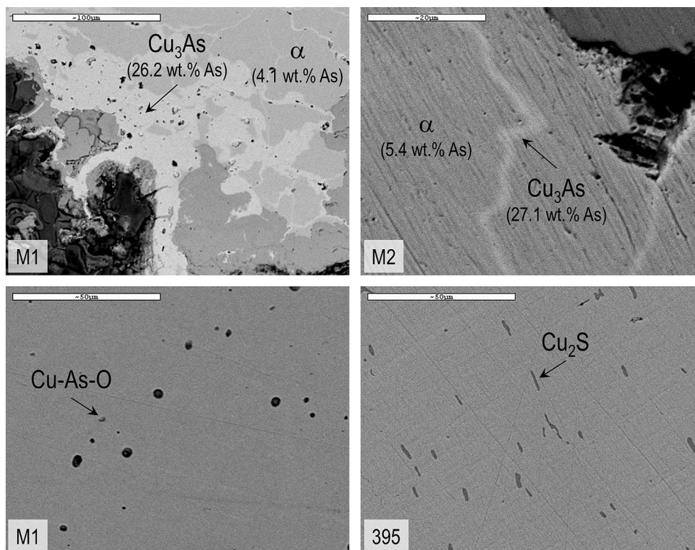
Fig. 4. SEM-BSE images and SEM-EDS spot quantifications of arsenical copper awls M1 and M2 from Monte da Cabida 3 and bronze awl 395 from Torre Velha 3.
