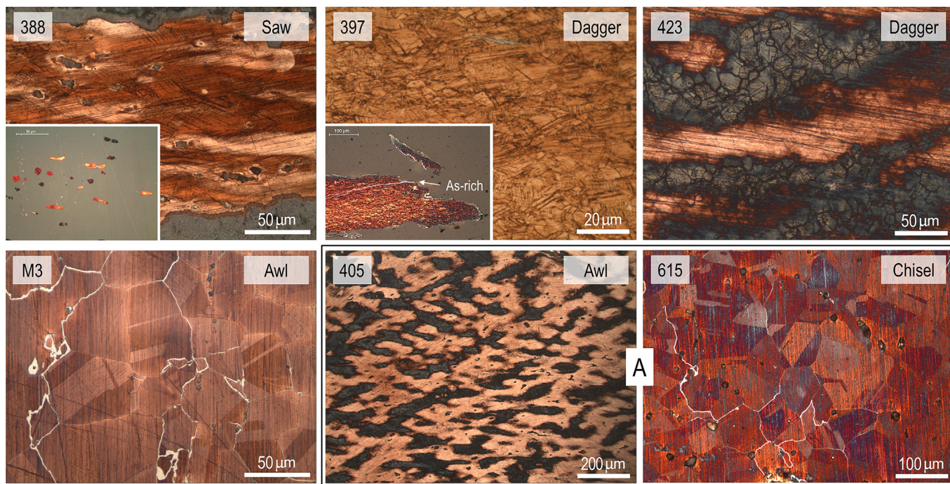
Fig. 3. Microstructures of MBA arsenical copper artefacts from Torre Velha 3 and Monte da Cabida 3 (A: unusual microstructures).
