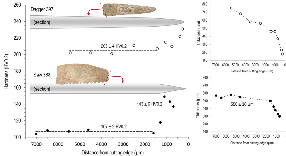
Fig. 6. Hardness and thickness profiles of MBA dagger 397 and saw 388 from Torre Velha 3.
