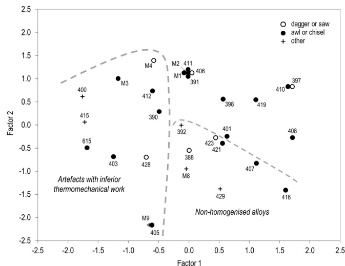
Fig. 8. Factor scores obtained from microstructural variables of MBA arsenical copper artefacts from Torre Velha 3 and Monte da Cabida 3 (artefacts 391, 406, 411, M1 and M2 have the same values).
