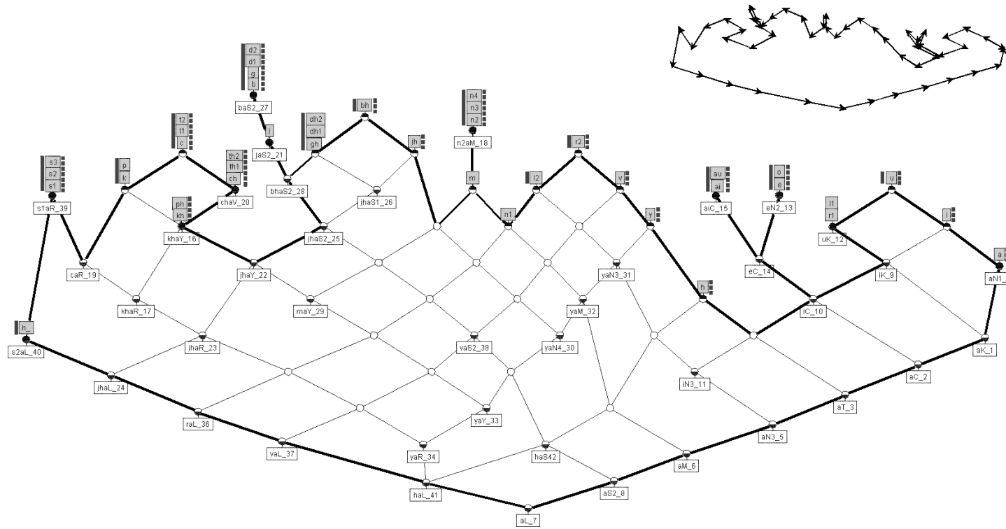
Figure 6: Hasse-diagram of the of the pratyāhāras used in the Aṣṭādhyāyī . The denotations in the figure are as follows: h_- is the duplicate of h and r1:r, l1:l, r2:r, l2:l, n1:ñ, n2:ṅ, n3:ṇ, n4:n, dh1:ḍh, dh2:dh, d1:ḍ, d2:d, th1:ṭh, th2:th, t1:ṭ, t2:t, s1:ś, s2:s, s3:s . The white boxes mark the 42 phonological classes which Pāṇini uses in the Aṣṭādhyāyī . The small figure on top shows the path in the S-graph which one has to choose in order to construct Pāṇini's Śivasūtras .
